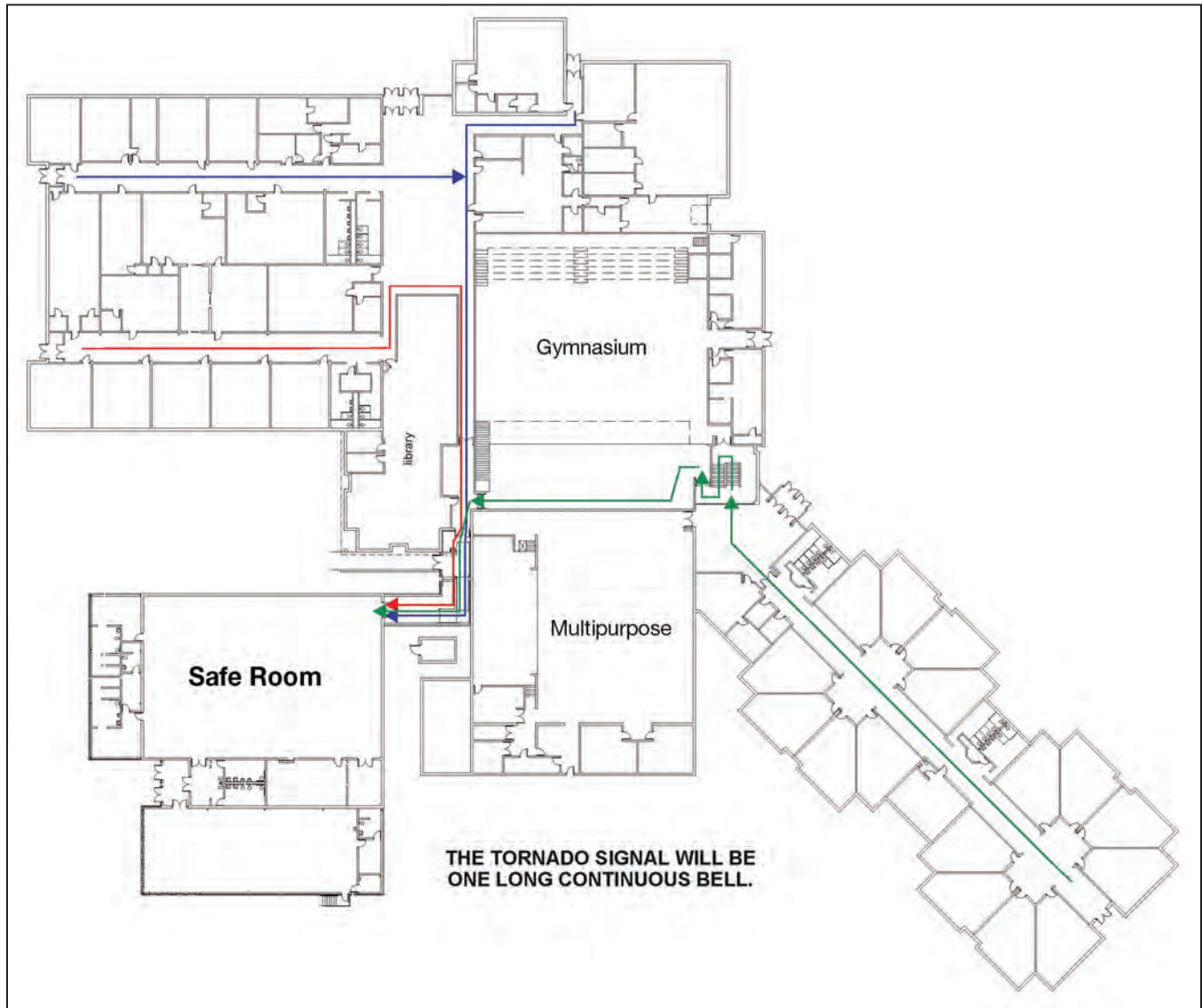
Figure A4-4. Example of a site plan clearly identifying safe room access routes
