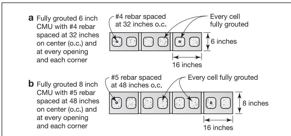
Figure B8-18. CMU wall assemblies
