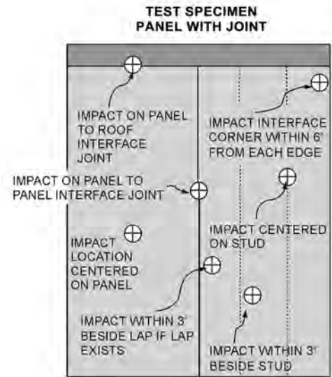
Figure B8-16. Impact test locations for a panel or framed roof or wall assembly (SOURCE: ICC 500 FIGURE 804.9.1(2); USED WITH PERMISSION)
