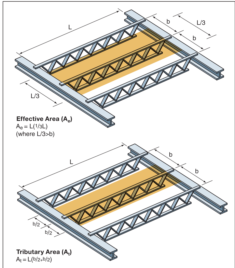
Figure B3-3. Comparison of tributary and effective wind areas for a roof supported by open-web steel joists
