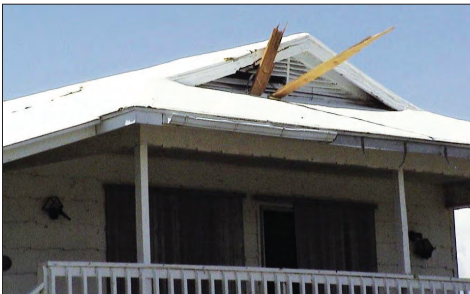
Figure B8-12. Impact of structural wood members in the gable end from a neighboring house (Pine Island, FL) (SOURCE: FEMA P-488)
