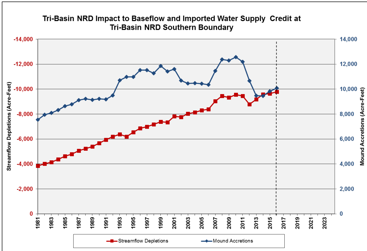
Figure 1: Modeled annual streamflow depletions and mound accretion for calendar years 1981 through 2016. The data in this figure were calculated using the August 2016 RRCA accounting procedures. In order to show both streamflow depletions and mound accretions for comparison in one chart, the negative values on the left vertical axis pertain to the red line, representing stream depletion values, and positive values on the right vertical axis pertain to the blue line, representing mound accretions.
