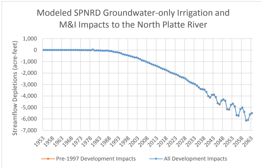
Figure 8. Modeled SPNRD streamflow impacts to the North Platte River from all groundwater-only irrigation and municipal and industrial (M&I) development with offsetting management actions and the streamflow impacts from development pre-1997.
