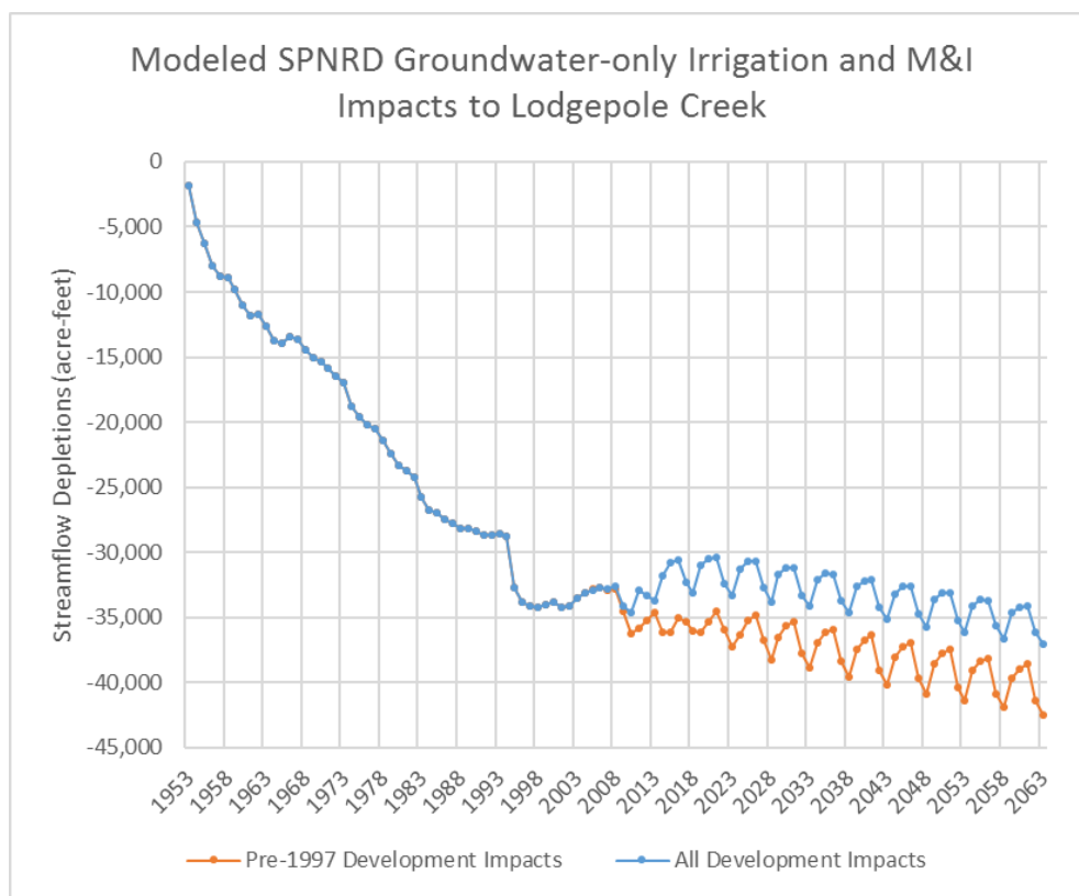
Figure 10. Modeled SPNRD streamflow impacts to the Lodgepole Creek from all groundwater-only irrigation and Municipal and Industrial (M&I) development with offsetting management actions and the streamflow impacts from development pre-1997.
