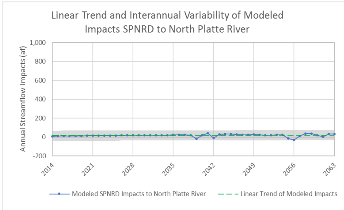
Figure 5. Modeled SPNRD Post-1997 impacts to the North Platte River, the linear trend line of the modeled impacts from 2014-2063, and the inter-annual variability range of modeled impacts across the trend.
