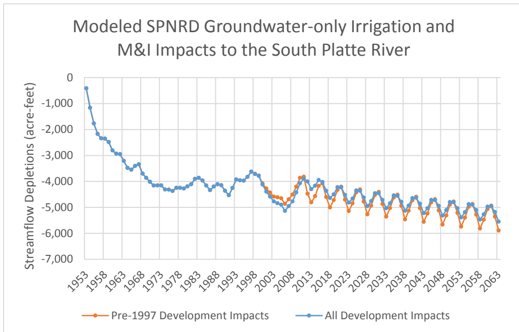
Figure 9. Modeled SPNRD streamflow impacts to the South Platte River from all groundwater-only irrigation and Municipal and Industrial (M&I) development with offsetting management actions and the streamflow impacts from development pre-1997.
